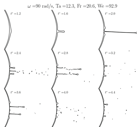
Simulation of the thin film instability which grows the surface of a rotating sphere and develop into fluid ligaments which eventually break-up into droplet for different flow conditions (simulation by Dr Bradley Boyd).
