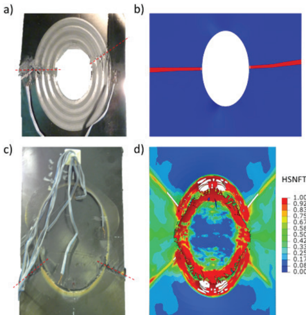
Failure modes of high stiffness scarfed elliptical hole panels: (a) SH test, (b) SH FEA prediction, (c) RH test, and (d) RH FEA prediction, showing Hashin fibre failure criterion in the longitudinal 0° ply.
